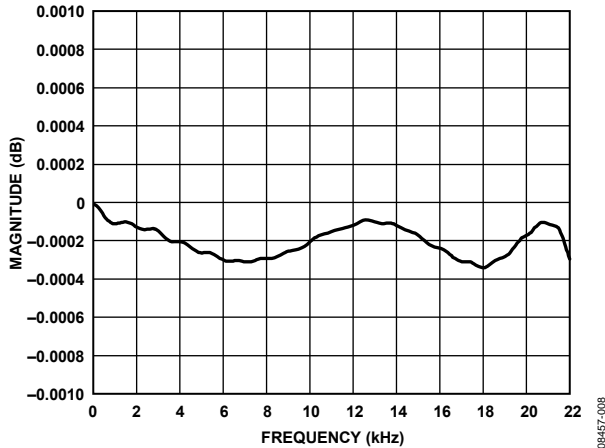
Figure 8. Pass-Band Response 8x Mode, 48 kHz Sample Rate
