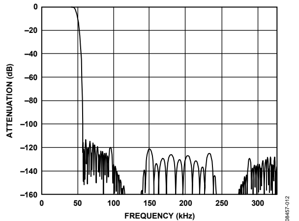
Figure 12. Complete Response, 4x Mode, 96 kHz Sample Rate
