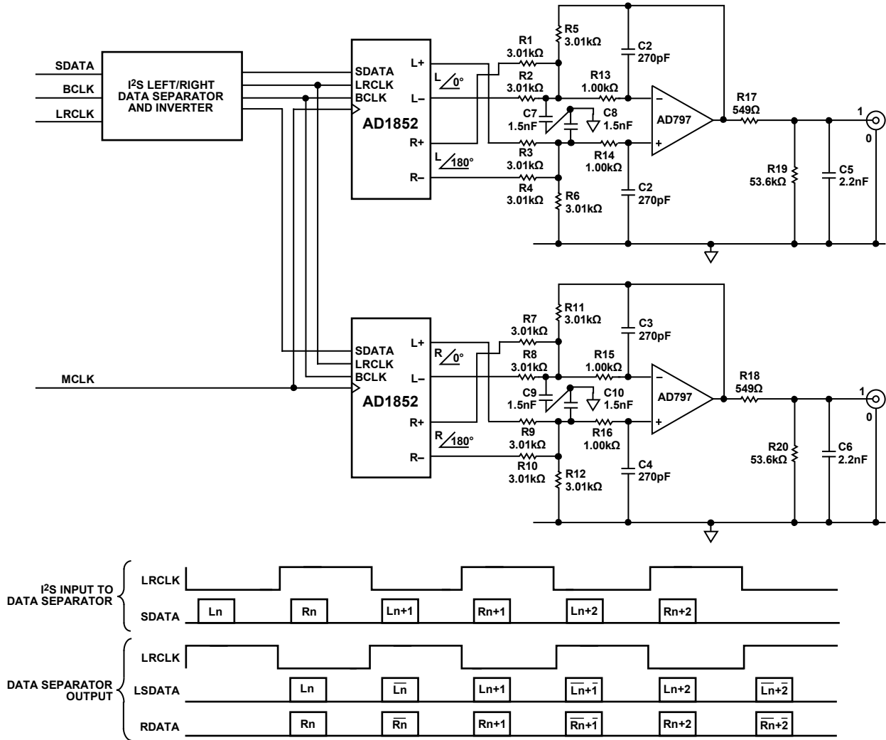
Figure 30. Mono Application Circuit
