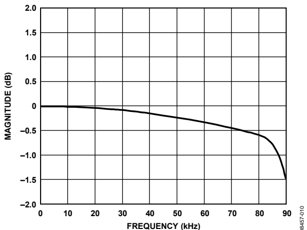
Figure 10. 88 kHz Pass-Band Response 2x Mode, 192 kHz Sample Rate
