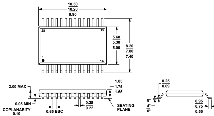
Figure 31. 28-Lead Shrink Small Outline Package [SSOP] (RS-28)
