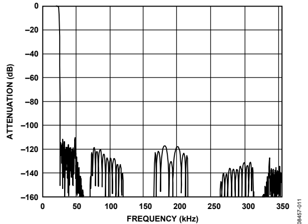
Figure 11. Complete Response, 8x Mode, 48 kHz Sample Rate
