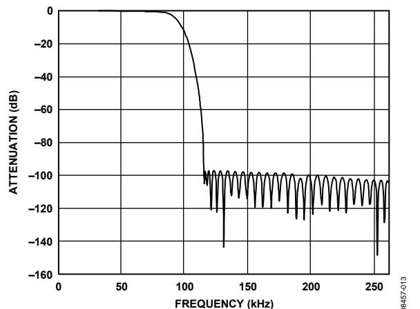
Figure 13. Complete Response, 2x Mode, 192 kHz Sample Rate
