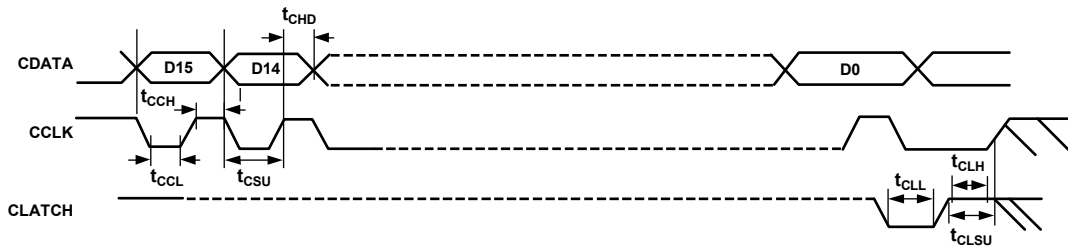
Figure 27. Serial Control Port Timing
