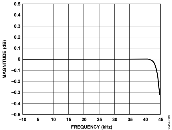
Figure 9. 44 kHz Pass-Band Response 4x Mode, 96 kHz Sample Rate
